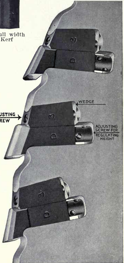
Section of Premier Metal Cutting Saw
