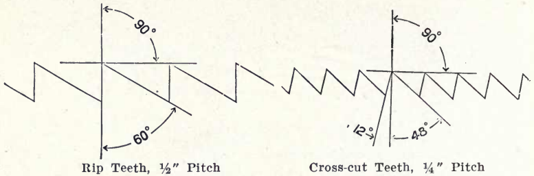
Rip Teeth, \frac{1}{2} " Pitch
