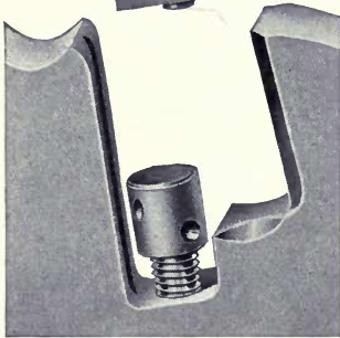
View of socket showing screw for regulating the height of tooth
