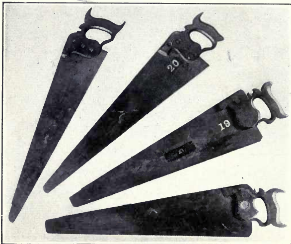
Early Types of Handsaws
